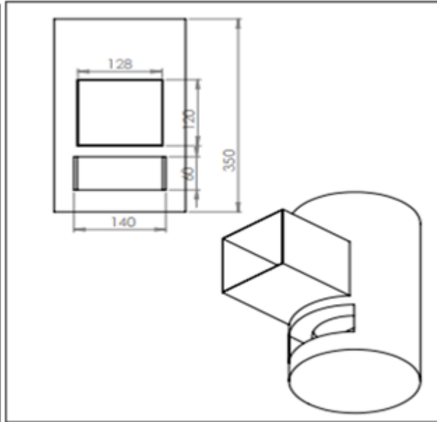
b) fuel magazine and air inlet
