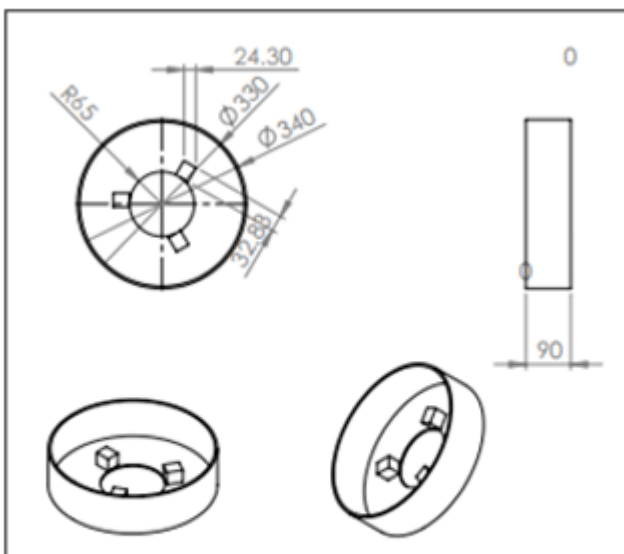
c) Pot skirt and pot rest
